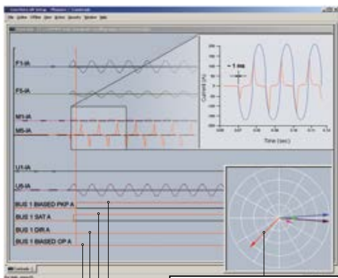
Despite heavy CT saturation the external fault is seen in the opposite direction
