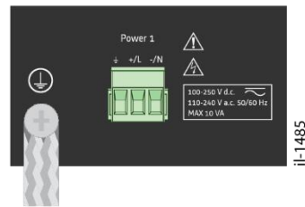
Figure 8: RT411 Grounding Strap
