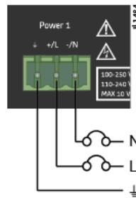
Figure 7: RT411 power connection
