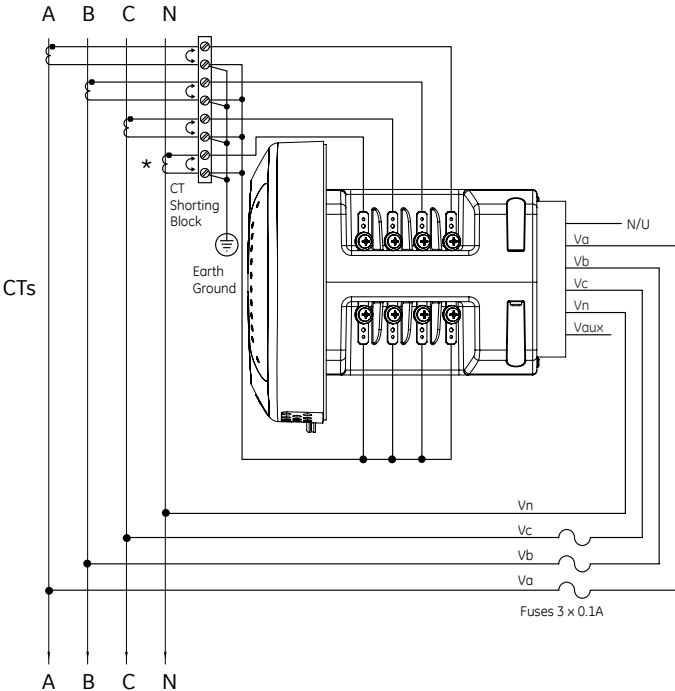
4-Wire Wye, 3 Element with 4 CTs and no PTs *Note: Optional CT for Current Measurement Only
