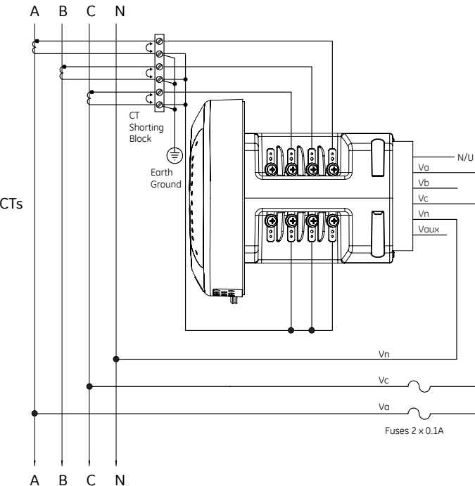
3-Wire, 2 Element Delta Direct with 2 CTs
